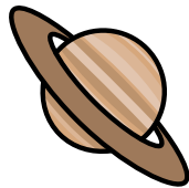
Saturn
