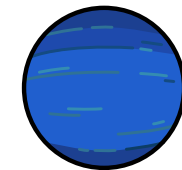
Neptune
